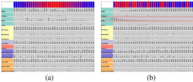
Fig. 6. Sorting columns. a) normally, columns are sorted by the distances of their corresponding clusters to the focal point. The closer the clusters are to the focal point, the closer the column is to the middle of the screen (and more red in color); b) the user can also sort the columns based on a specific data dimension.
