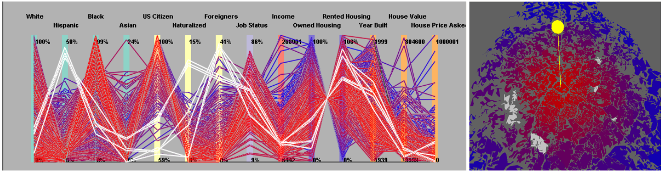
Fig. 8. Case study 1: Finding neighborhoods with high Hispanic population near the downtown area: (right) the user starts by putting the focal point over the downtown region; (left) using brushing in the parallel coordinates window, the user highlights the regions that have high Hispanic population. Notice the positive correlation between the Hispanic population, the percentage of foreigners, and the percentage of residents who rent their housing in these selected areas.
