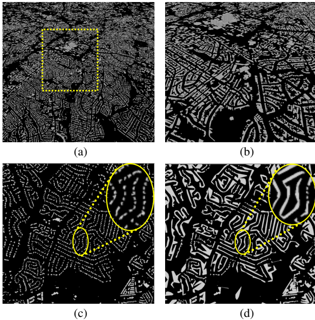
Fig. 1. The building model aggregation used by UrbanVis. a) View of downtown Charlotte and its surrounding regions from afar; b) what is actually being rendered when the selected yellow box region is enlarged; c) using a pixel tolerance \epsilon of 50; d) setting \epsilon to 500: notice that as \epsilon increases, so does the amount of aggregation. This results in larger, but fewer, clusters.
