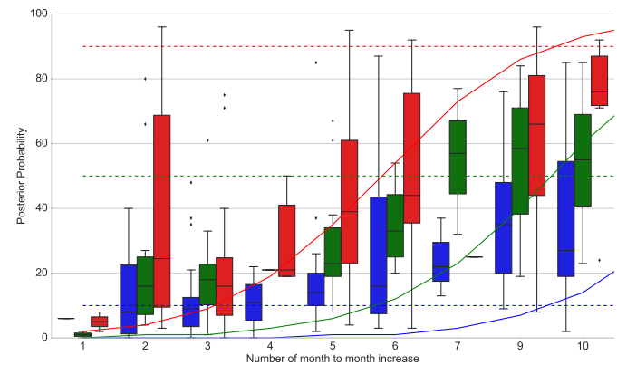
Fig. 5. A visualization of difference by the prior of the probability of the company being "strong", red is 0.9, green is 0.5, and blue is 0.1. The dashed lines show priors, the continuous lines show the Bayesian posterior (which could be calculated with the prior, the data, and the likelihoods), and the scatter plot shows the responses of the user on the y axis against the data they've seen, represented by the number of month to month increases.
