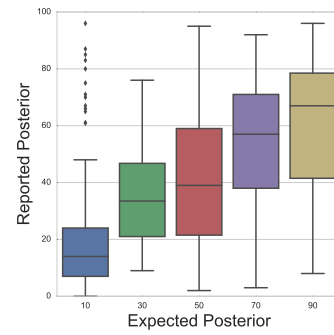
Fig. 4. Box plot of the responses against expected answer bucketed into groups of step size of 10%, pooling both visualization types.
