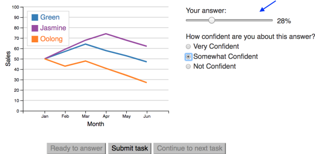
Fig. 3. Experiment design overview, including the simple visualization of the prior and the fixed conditional probability information, and the response collection interface.
