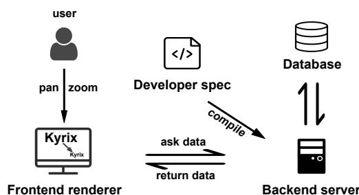
Figure 2: Kyrix system architecture.
