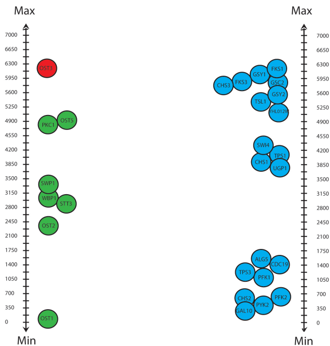
Fig. 7. A BPM from Kelley and Ideker not validated by our method. This BPM illustrates clustering of subsets of genes within the compensatory pathway.
