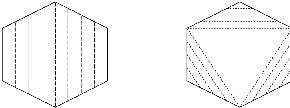
Figure 8: Stronger lower bounds: families of paths
