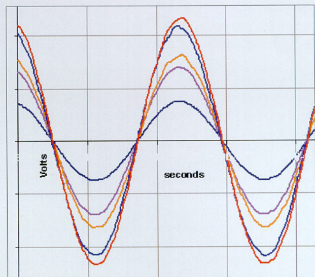
Fig. 14. A 20kHz sine wave is applied to the spiral's inner section (dark blue). As the probe is placed across more of the spiral, the signal voltage rises (lavender to red). Vertical: 2V/div. Horizontal: .1ms/div.
