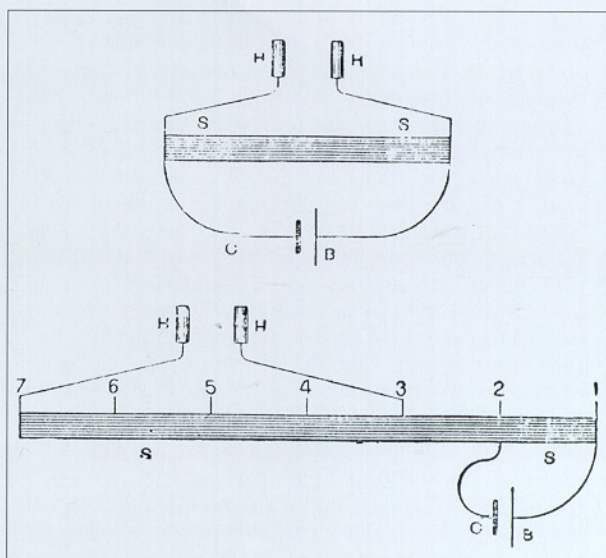
Fig. 4. Unwound spirals of Henry (top) and Page (bottom), with shock handles (HH), battery (B) and Page's numbering of the intermediate tabs (Fleming 1892.)
