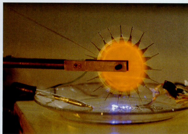
Fig. 10. Purple sparks show in time exposure plus flash of my star wheel (pulled by string on left) through galinstan. Photo Jeff Tinsley.
