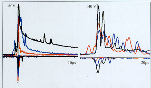
Fig. 16. Overlay plots of maximal and minimal envelopes produced in runs consisting of 256 induced events. Left: Red – For this run, battery current, a resistor (as a body model) and probe are placed across inner spiral segment; Blue – battery current, resistor and probe go midway across spiral; Black – battery current, resistor and probe are placed across whole spiral (peak is 80 V, time interval is 10 \mu s). Right: Red – battery current, resistor and probe are across inner spiral; Blue – battery current remains across inner spiral while probe and resistor go midway across it; Black – battery current remains across inner spiral while probe and resistor go across whole spiral (peak is 140V, time interval is 20 \mu s).
