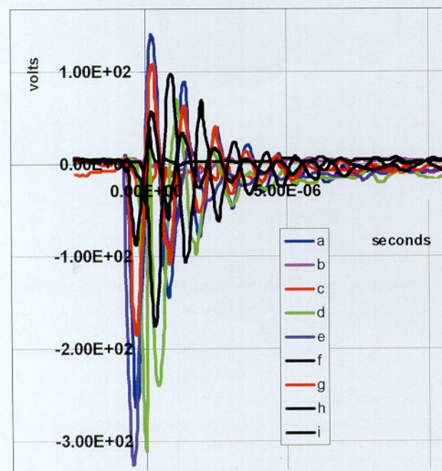
Fig. 13. Overlay of 9 voltage traces (a-i), induced successively in the spiral with star wheel interrupter; with no changes in circuit between events. Vertical: 100V/div. Horizontal: 5µs/div.
