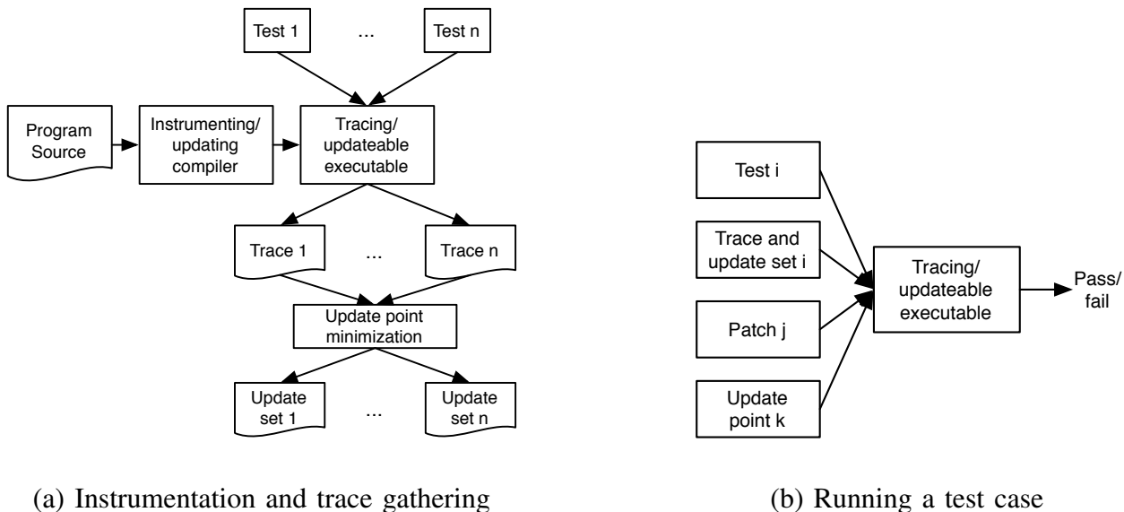
Fig. 2. DSU testing framework architecture
