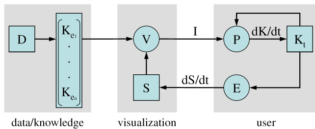
Figure 2: The refined model of the operational model in Figure 1 having the collections of explicit knowledge K_{e_1} to K_{e_n} .
