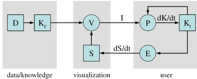
Figure 1: A model of knowledge-based visualization that integrates van Wijk's model [10] with explicit and tacit knowledge
