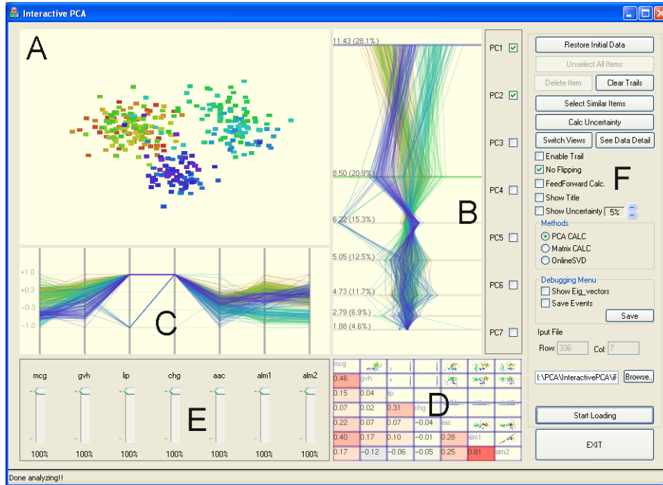
Figure 2: Showing the four views and the two control panels. (A) Projection view. Data items are projected onto the two user-selected eigenvectors (in this case, the primary and secondary principle components). (B) Eigenvector view. Each eigenvector is treated as a dimension in this parallel coordinates view, and every data item is drawn as a line. (C) Data view. Another parallel coordinates view, but this time each dimension represents the dimensions in the original data, and each line represents each data item. (D) Correlation view. Pearson-correlation coefficient and the relationships (scatter plot) between each pair of variables are represented. (E) Dimension sliders. Each slider controls the amount of contribution of a dimension in the PCA calculation. (F) Control options
