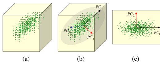
Figure 1: Illustration of principal component analysis.
