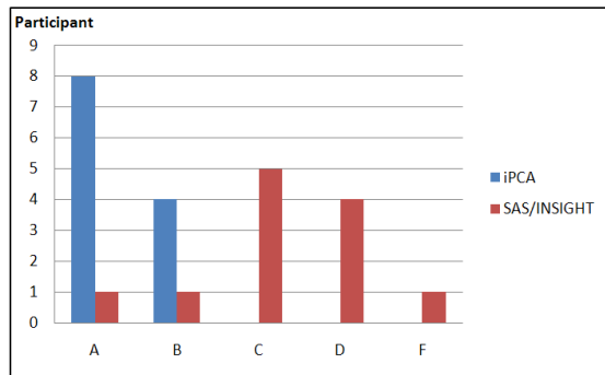
Figure 6: At the end of the evaluation, each participant grades the systems on a scale of 'A' to 'F'.
