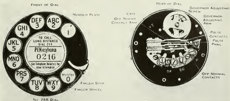
Fig. 6—Subscriber's Dial
