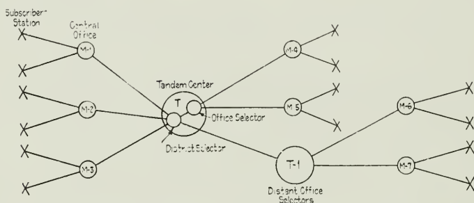
Fig. 27—Tandem Trunking Plan Showing Distant Office Selector
