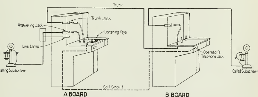
Fig. 4—Diagram Showing Manual Interoffice Connection
