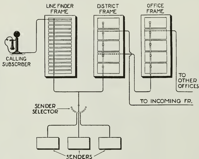
Fig. 13—Diagram of Line Finder, District and Office Frames
