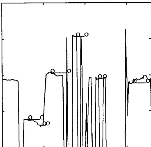
Figure 4. Result of applying the fixation recognition algorithm to the data of Figure 3. A horizontal line beginning and ending with an \circ marks each fixation at the time and coordinate position it would be reported.
