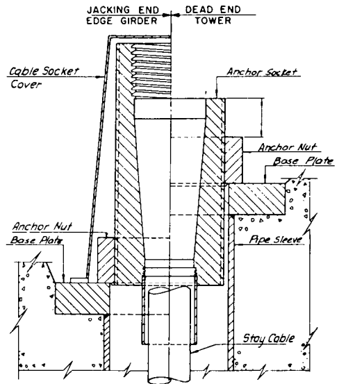
CABLE ANCHORAGE ASSEMBLY
