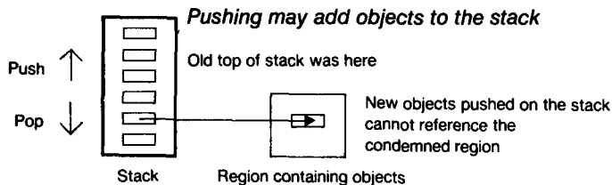
FIGURE 5. Scavenging the Stack.
