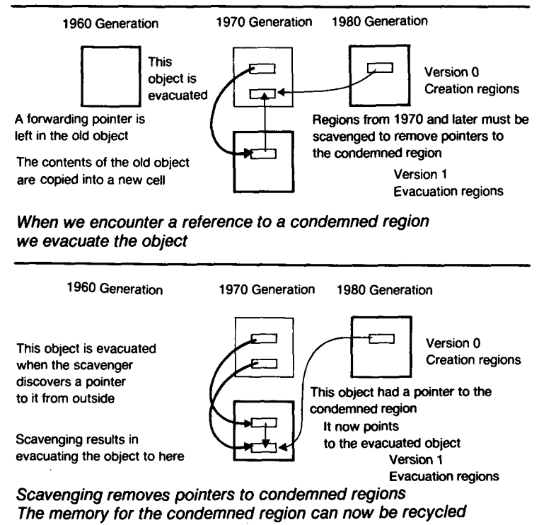
FIGURE 3. Evacuation and Scavenging.
