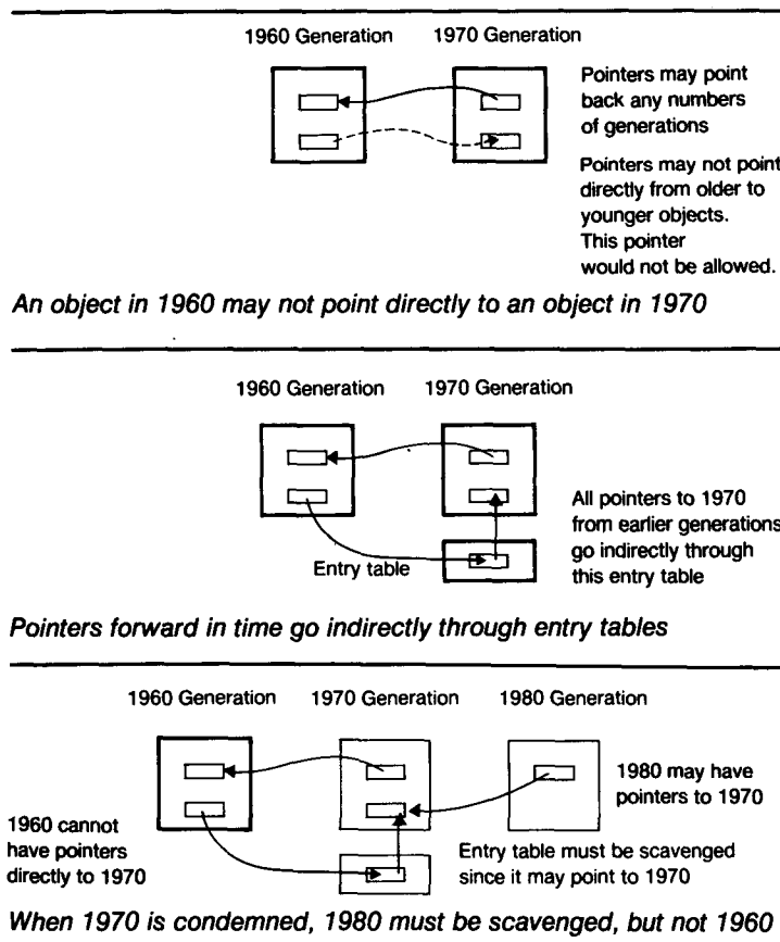
FIGURE 4. Entry Tables for Forward Pointers Reduce Scavenging.
