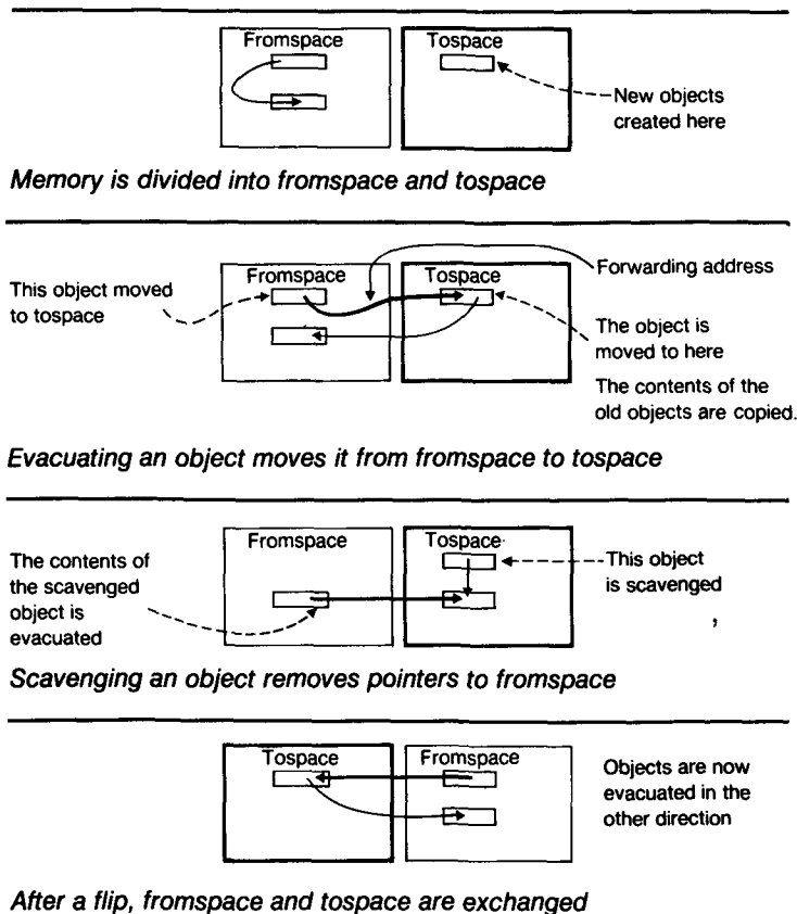
FIGURE 1. Henry Baker's Real-Time Garbage Collector.
