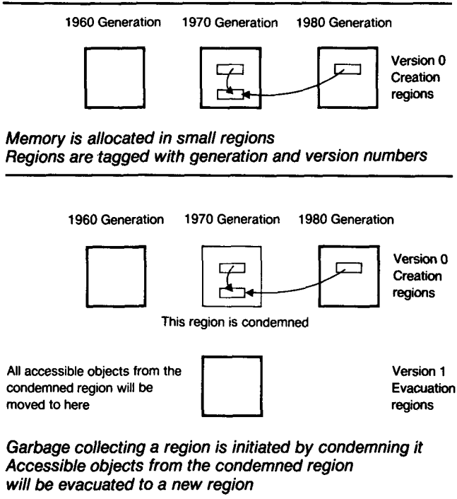
FIGURE 2. Our Real-Time Garbage Collector.
