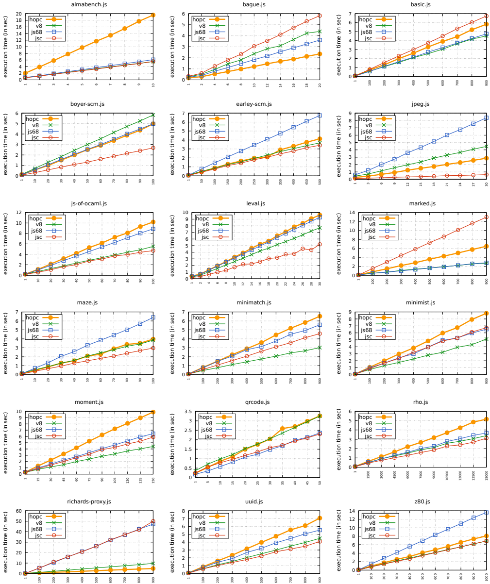
Fig. 9. JIT performances (V8 (6.8.275.32), Jsc (4.0), and Js68 (C68)) vs aot performances (hop). The vertical axis are the clock wall execution times. Smaller is then better. The horizontal axis are the numbers of iterations of the benchmark. Measures collected on Linux 5.3 x86_64, powered by an Intel Xeon E5-1650.
