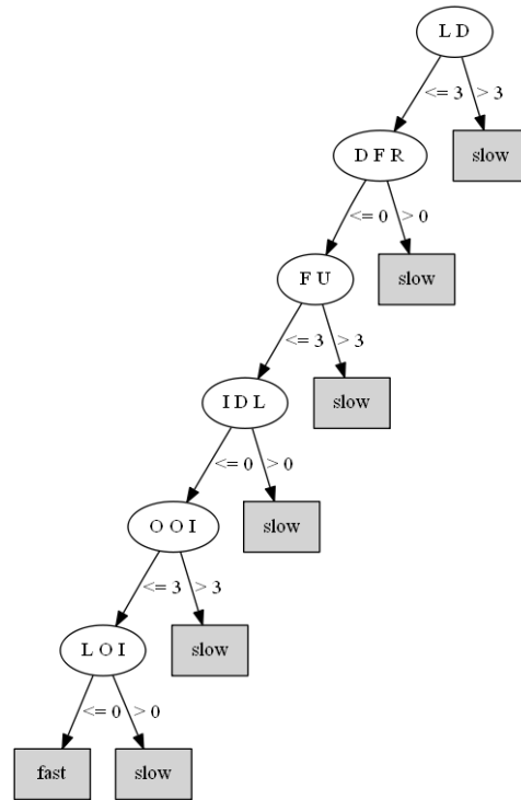
Fig. 3. This is the decision tree generated as a classifier for fast versus slow completion time with mean class splitting. Each internal node represents an individual decision to be made about a data point. The text within the node is the n-gram used to make the choice, and the labels on the out-edges indicate how to make the choice based on the count for a given data point of the n-gram specified. Leaf nodes indicate that a decision is made and are marked with the decided class.
