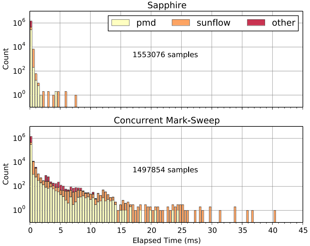
(a) Task times for Sapphire and Concurrent Mark-Sweep for applicable benchmarks (excluding eclipse , ijython , lusearch and xalan ). Each bar represents 500 \mu s.
