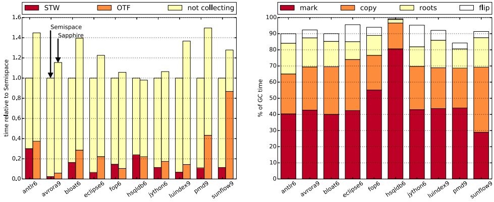
(a) Visualisation of execution times from Table 6 where the first column per pair represents Semispace execution times and the second Sapphire.
