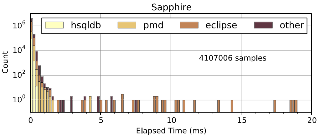
(b) Task times for Sapphire including eclipse , ijython . 'Other' excludes lusearch and xalan . Note that the bars are stacked, giving more visual weight to hsqldb than to 'other'.
