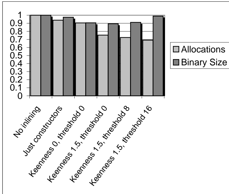
Fig. 2. Effect of inlining threshold on allocations and binary size.
