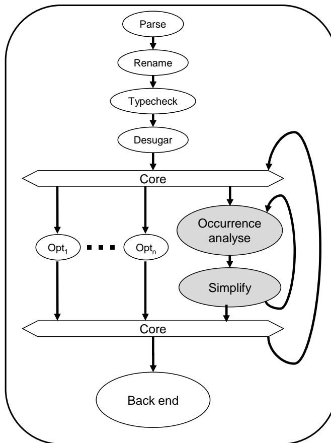
Fig. 1. Overall structure of GHC.
