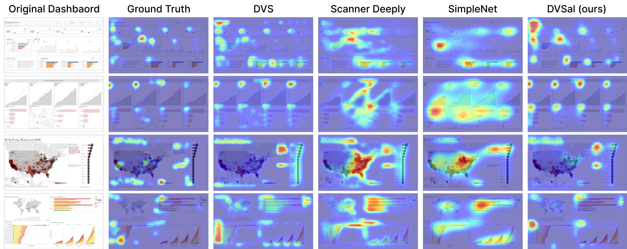
Fig. 9. The qualitative comparison of DVSal with other methods. DVSal predicts saliency maps more accurately compared to DVS [20], Scanner Deeply [21], and SimpleNet [27], effectively distributing visual attention across all visual objects.
