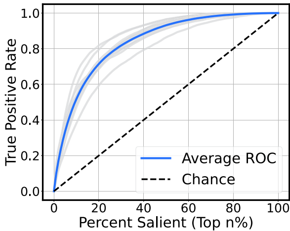
Fig. 3. ROC curve measured for the 16 DVELite dashboards viewed by 60 participants. Gray lines depict individual dashboards, while the blue line represents the average ROC curve.
