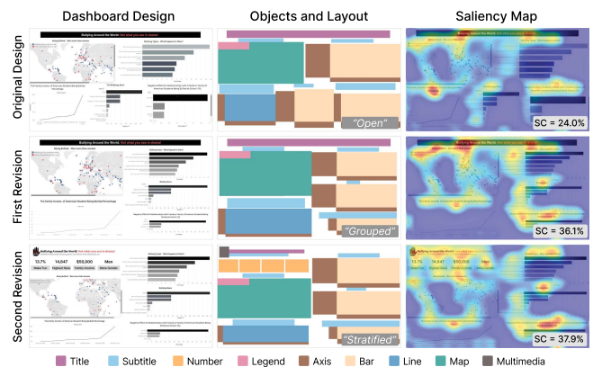
Fig. 10. The original dashboard design (top) and two revisions (middle and bottom). The saliency coverage (SC) of the improved designs increased by 12.1% and 1.8%, respectively.
