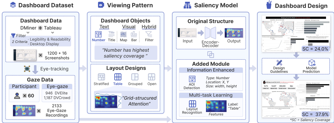
Fig. 1. Pipeline of the dashboard vision study. We assemble a dataset of 1,216 dashboards (from DMiner [26] and Tableau), including labels for dashboard objects and eye-movement data. This dataset supports the analysis of viewing behavior and the development of a saliency model to inform and guide dashboard design.
