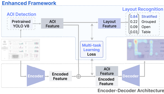
Fig. 8. Overview of DVSsal network. An AOI detection module and a layout recognition module are integrated into the encoder-decoder architecture. A multi-task learning mechanism is further adapted to collectively train the entire network.
